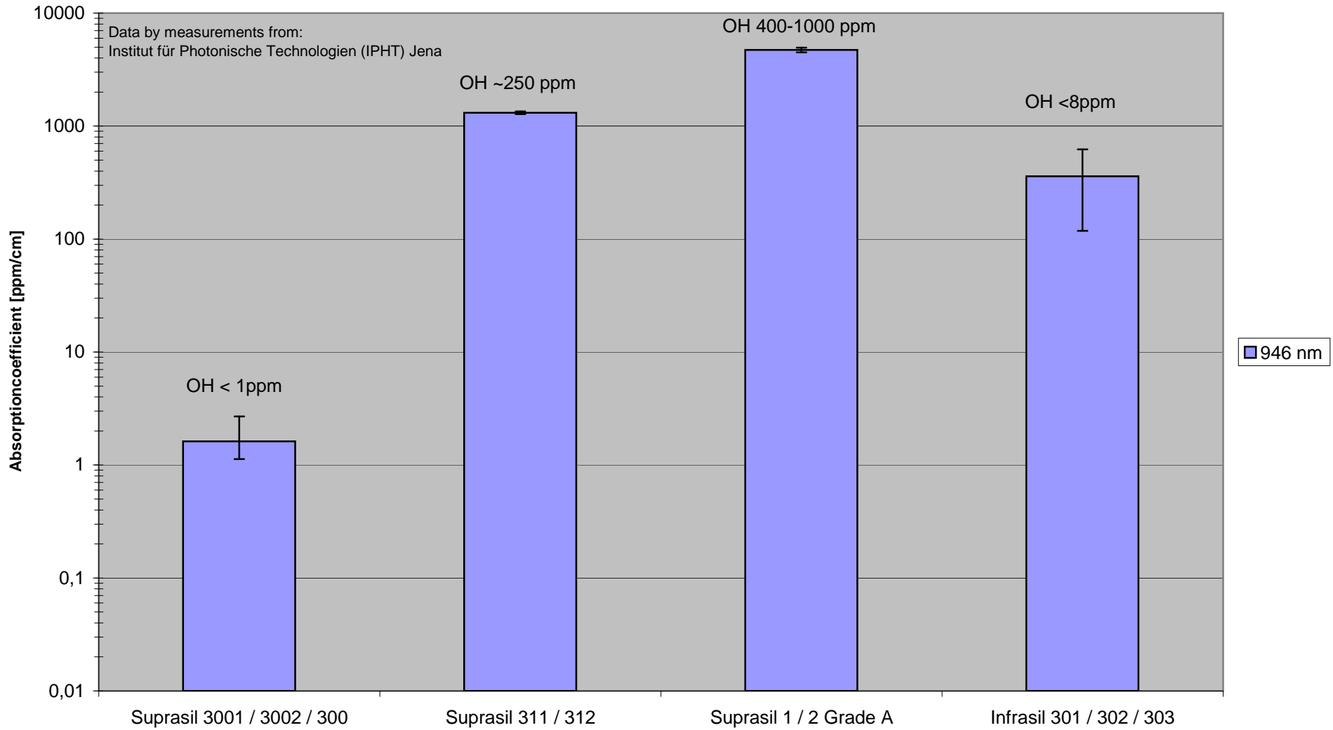
Typical Absorption of different Heraeus Material Grades @ Wavelength = 946nm
